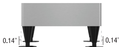
Bin Flanged Legs: B/BD-300SF
