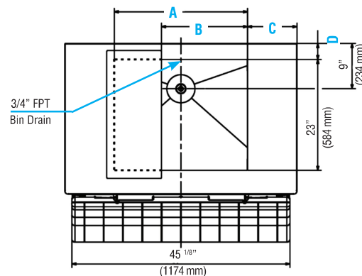
TOP VIEW B-1150/1300/1500/1650SS
