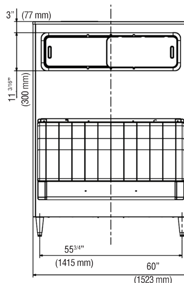
FRONT VIEW B-1500/1650SS
